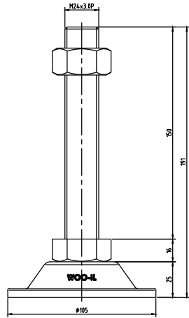
BL105-M24-150
