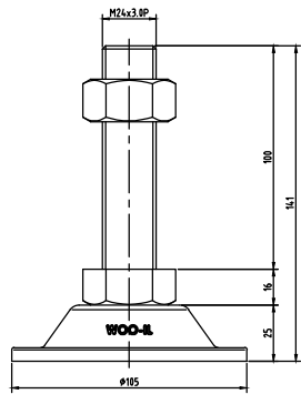
BL105-M24-100
