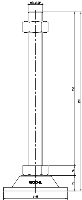
BL105-M24-250
