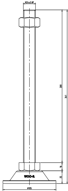
BL105-M24-300
