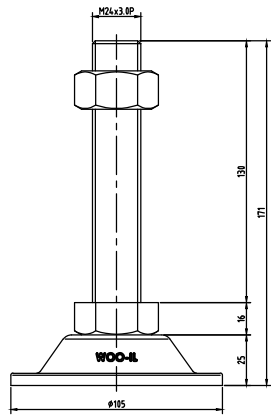
BL105-M24-130
