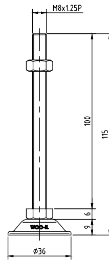
BL36-M8-100
