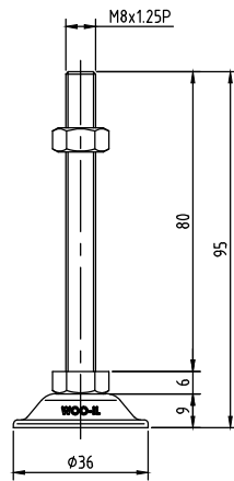
BL36-M8-80
