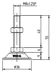
BL36-M8-40
