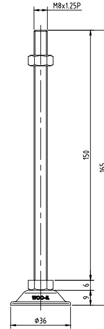
BL36-M8-150
