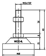
RL68-M12-50
