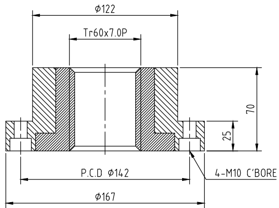
FI-TYPE
