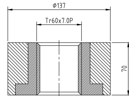
W-TYPE (용접형)
