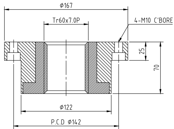
FP-TYPE
